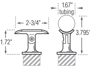
Dimensions for Adjustable Saddle (Round)
