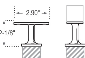
Dimensions for Fixed Saddle (Flat)
