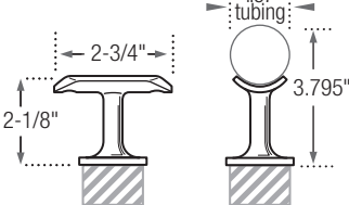
Dimensions for Fixed Saddle (Round)
