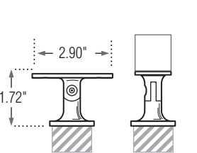
Dimensions for Adjustable Saddle (Flat)
