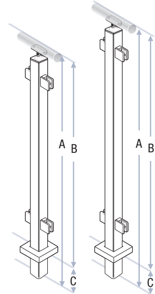
36-inch Post
