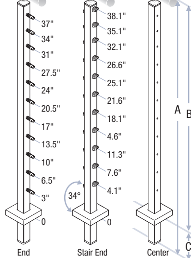
42-inch Post
