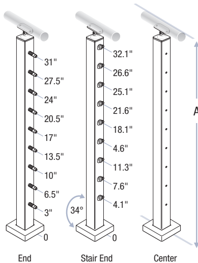
36-inch Post
