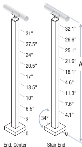
36-inch Post
