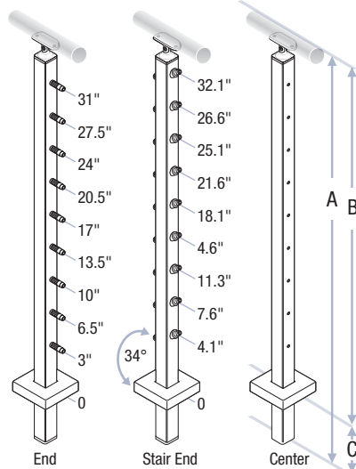
36-inch Post
