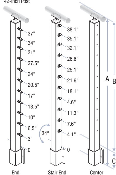
42-inch Post
