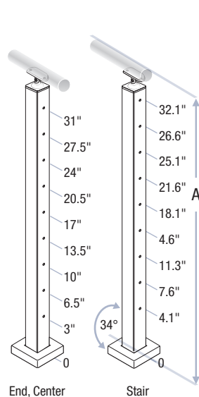
36-inch Post
