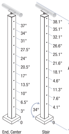
42-inch Post
