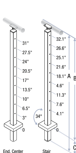
36-inch Post
