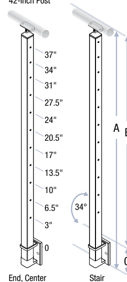
42-inch Post
