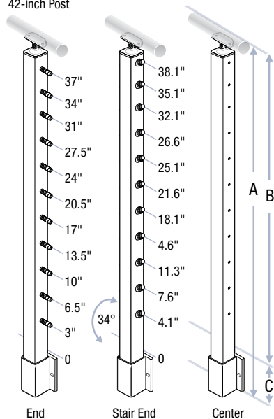
42-inch Post
