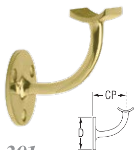
301 Standard Handrail Bracket
